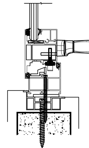
A SECTION DETAIL
