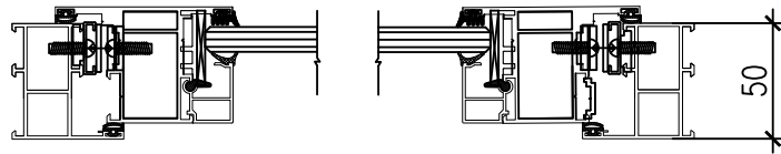
B SECTION DETAIL
